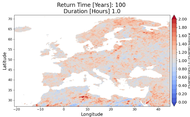
Fig. 3 KOSTRADAMUS output over Europe for the IFS NEMO run.
